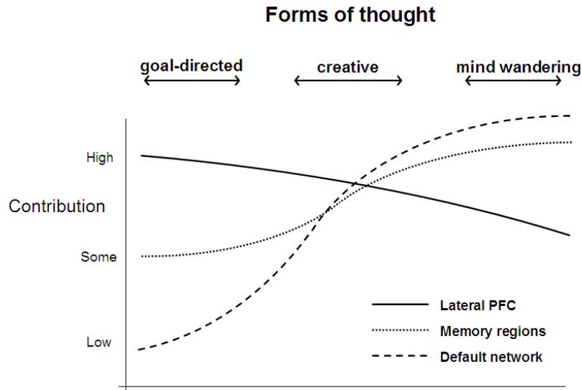
Figure 2. Proposed relative contribution of the lateral PFC, temporal lobe memory regions and the default network to goal-directed, creative, and spontaneous thought.
